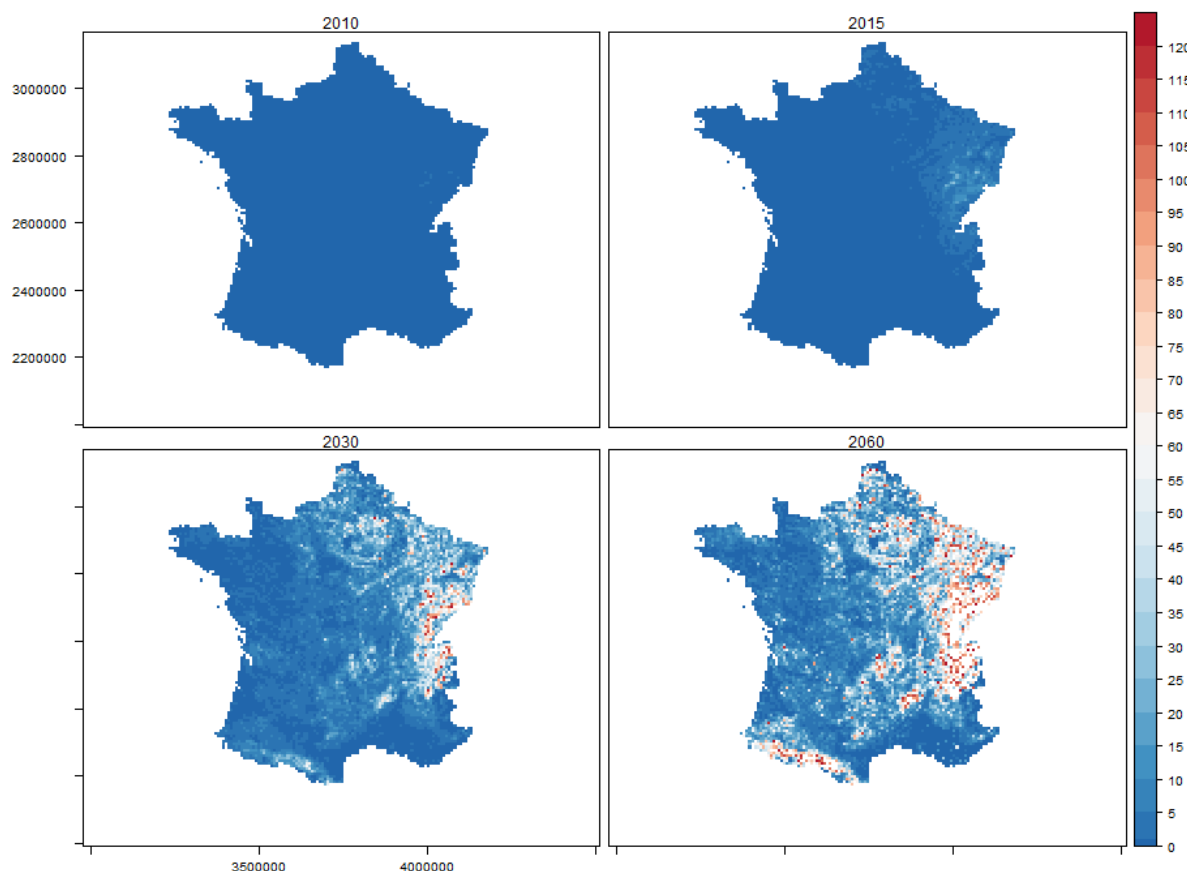
FIGURE: Ash dieback impacts: Common ash ( Fraxinus excelsion ) expected standing volume losses (cubic metres per hectare, resolution 8x8 km)
